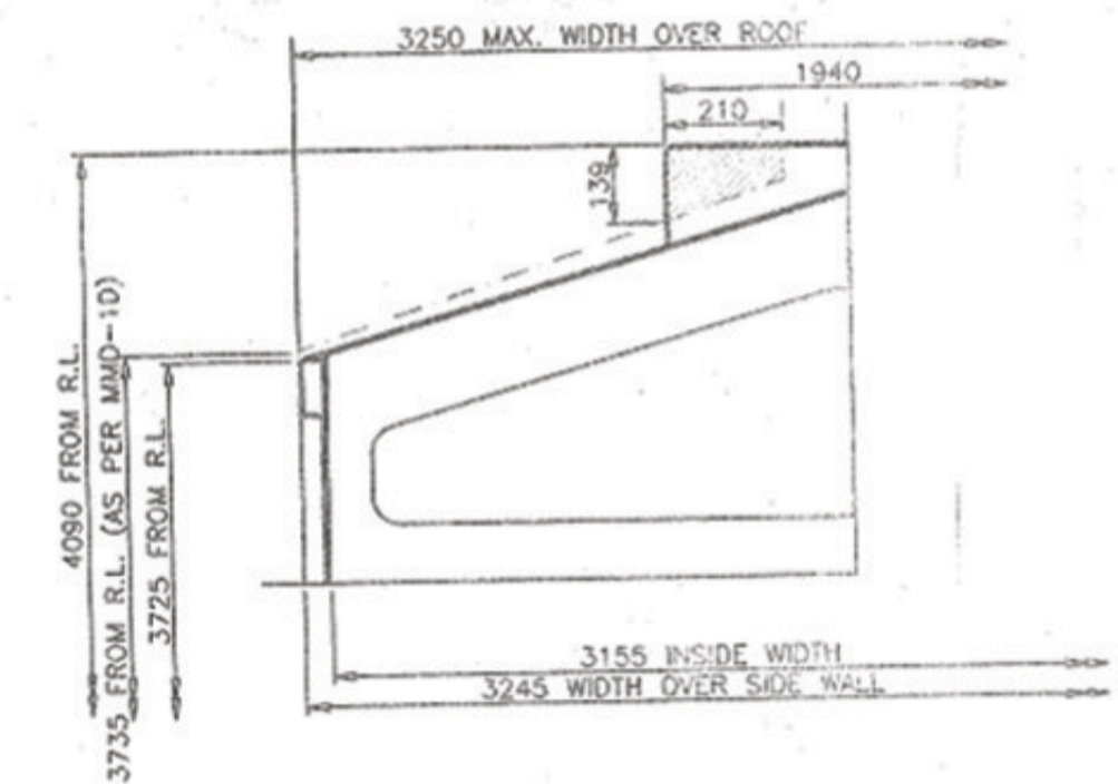
DETAIL AT 'X' INFRINGEMENT DETAILS
